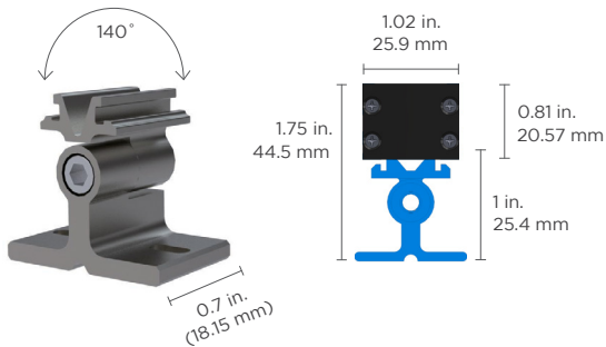
Tilttable Stand For adjustable mounting angles
