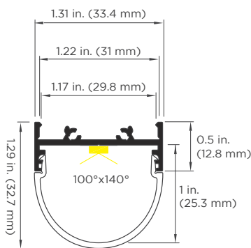
Width: 1.31 in. (33.4 mm) Height: 1.29 in. (32.7 mm) Internal Width: 1.22 in. (31 mm) Internal Height: 1 in. (25.3 mm)
