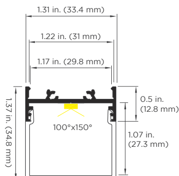
Width: 1.31 in. (33.4 mm) Height: 1.37 in. (34.8 mm) Internal Width: 1.22 in. (31 mm) Internal Height: 1.07 in. (27.3 mm)
