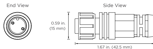
Molded Power Feed End Cap Side Feed
