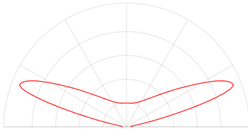
400 Series Batwing Beam Pattern
