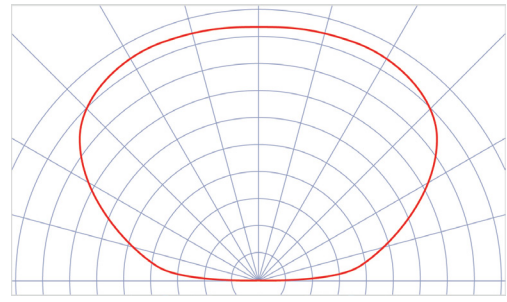
L4 Beam Pattern
