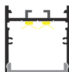
WH35 W: 1.37 in. / 35 mm H: 1.47 in. / 37.5 mm Inside W: 1.23 in. / 31.2 mm
