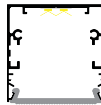
AS53 W: 2.09 in. / 53 mm H: 2.09 in. / 53 mm Inside W: 1.32 in. / 33.6 mm Inside H: 2 in. / 51 mm
