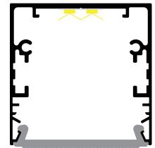
AS53 W: 2.09 in. / 53 mm H: 2.09 in. / 53 mm Inside W: 1.52 in. / 38.6 mm Inside H: 2 in. / 51 mm
