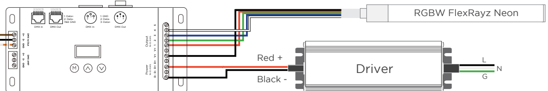
5 Channel DMX Interface Part #: DMXINFOLED5
