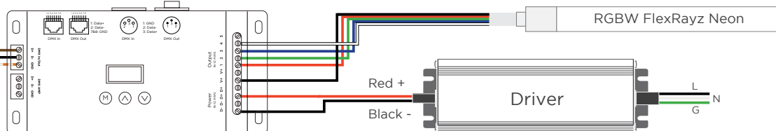
5 Channel DMX Interface Part #: DMXINFOLED5
