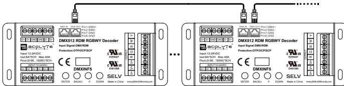
RJ45 connected in parallel
