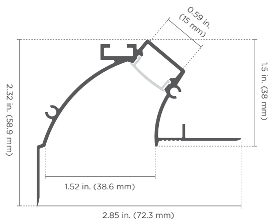
Overall Width: 2.85 in. (72.3 mm) Visible Width: 1.52 in. (38.6 mm) Height: 2.32 in. (58.9 mm) Internal Width: 0.59 in. (15 mm)
